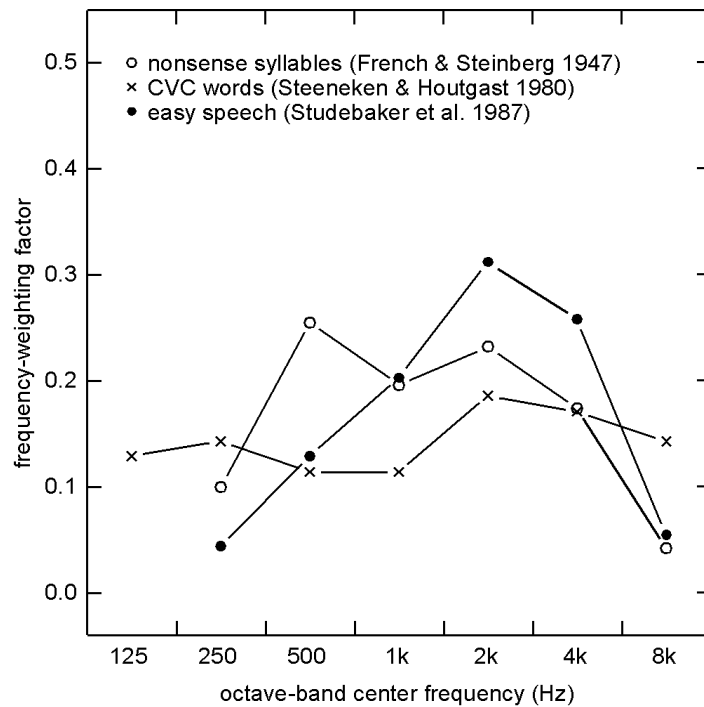
Fig.8. Frequency weighting functions for the AI and STI after French and Steinberg (1947), Steeneken and Houtgast (1980), and Studebaker et al. (1987).
