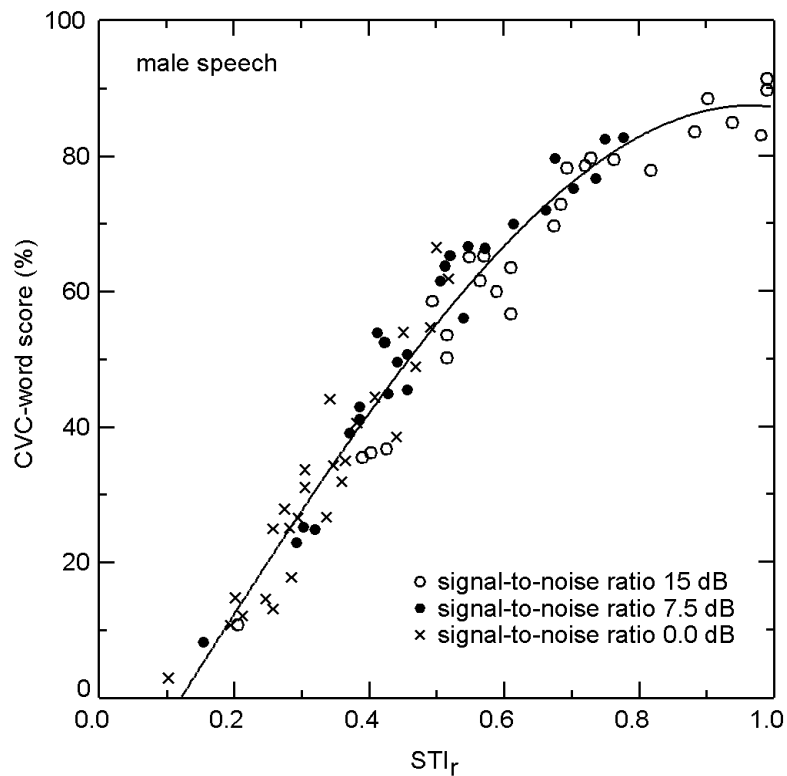
Fig.2. Relation between the STI_r and the CVC-word score for the 78 conditions involving MALE speech. The standard deviation, representing the vertical spread around the best-fitting third-order polynomial is s = 4.7\% .
