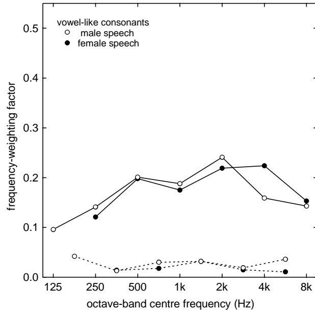
Fig.11. Frequency-weighting factors for the octave-band contribution \alpha_k (solid line) and redundancy correction \beta_k (dashed line) for the VOWEL-LIKE consonants and for the male and female speech.
