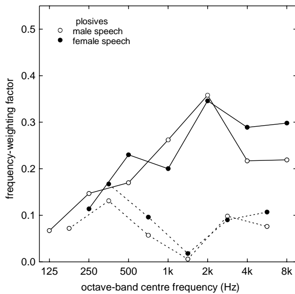
Fig.10. Frequency-weighting factors for the octave-band contribution \alpha_k (solid line) and redundancy correction \beta_k (dashed line) for the PLOSIVES and for the male and female speech.
