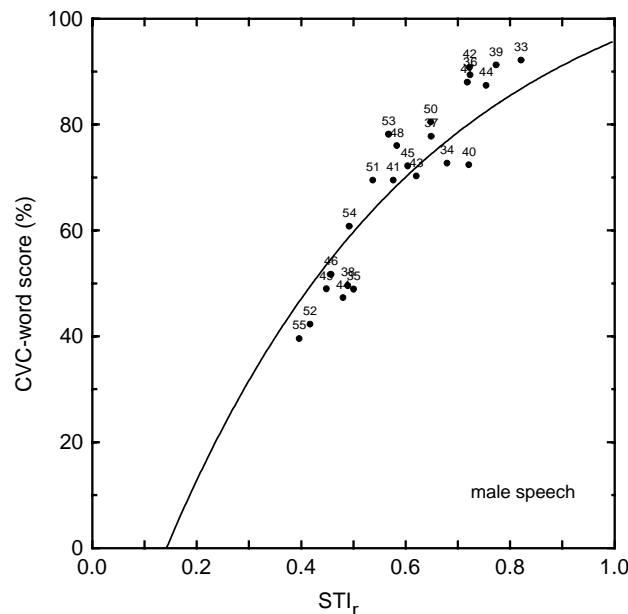
Fig. 18 Relation between the STI_r and the CVC-word score for the 24 communication channel conditions including distortion in the time domain for MALE speech. The standard deviation, representing the vertical spread around the predefined polynomial is s = 6.9\% .
