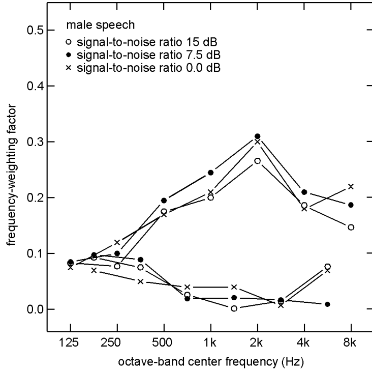
Fig.5. Frequency-weighting factors \alpha_k (upper curves) and redundancy-correction factors \beta_k (lower curves) for the MALE conditions at three signal-to-noise ratios as given in Fig. 6.
