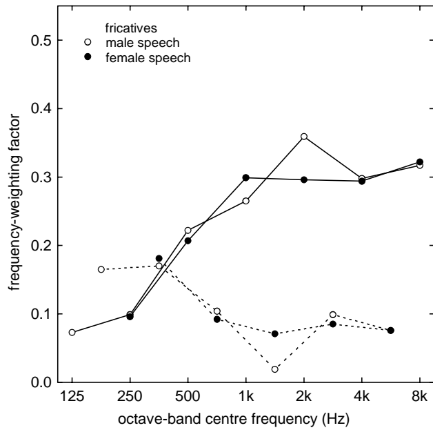
Fig. 9. Frequency-weighting factors for the octave-band contribution \alpha_k (solid line) and redundancy correction \beta_k (dashed line) for the FRICATIVES and for the male and female speech.
