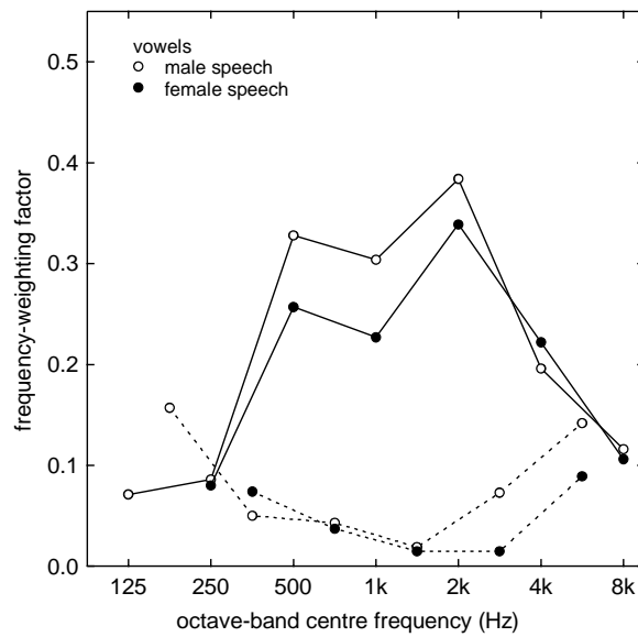
Fig. 12. Frequency-weighting factors for the octave-band contribution \alpha_k (solid line) and redundancy correction \beta_k (dashed line) for the VOWELS and for the male and female speech.
