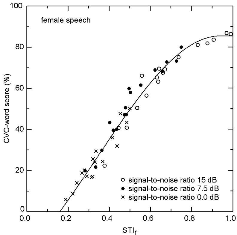
Fig.3. Relation between the STI_r and the CVC-word score for the 51 conditions involving FEMALE speech. The standard deviation, representing the vertical spread around the best-fitting third-order polynomial is s = 4.2\% .
