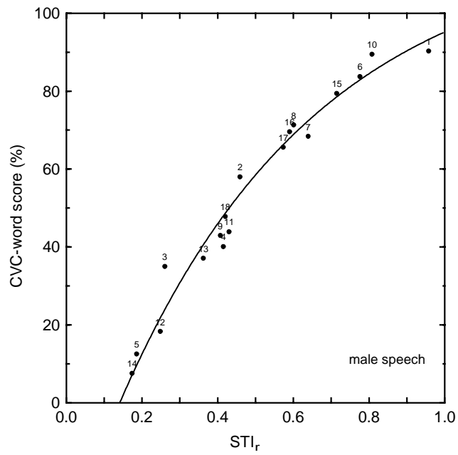
Fig. 15 Relation between the STI_r and the CVC-word score for the 18 transfer conditions including band-pass limiting and noise for MALE speech. The standard deviation, representing the vertical spread around the predefined polynomial is s = 4.4\% .
