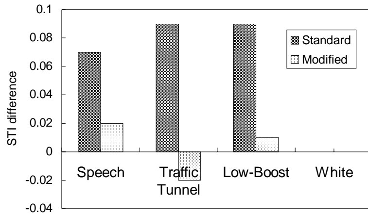
Fig.7. Differences in STI between 75 and 105 dBA (standard and modified model) based on male SRT results (2 talkers, 4 listeners).
