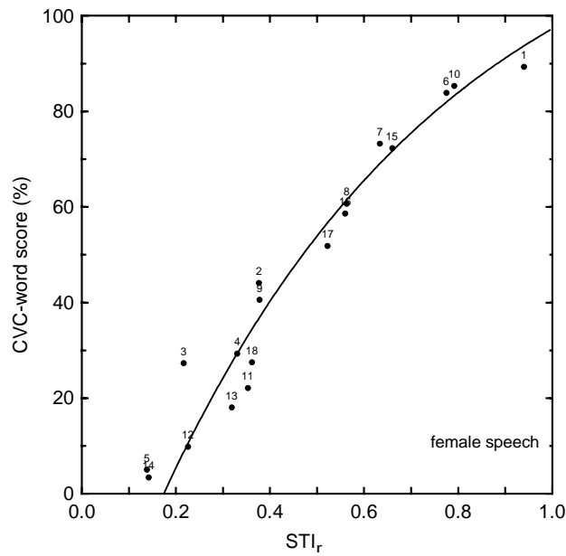
Fig. 16 Relation between the STI_r and the CVC-word score for the 18 transfer conditions including band-pass limiting and noise for FEMALE speech. The standard deviation, representing the vertical spread around the predefined polynomial is s = 6.6\% .
